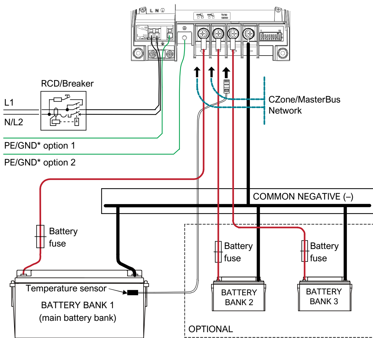
Figure 3: Installation drawing of the ChargeMaster Plus
