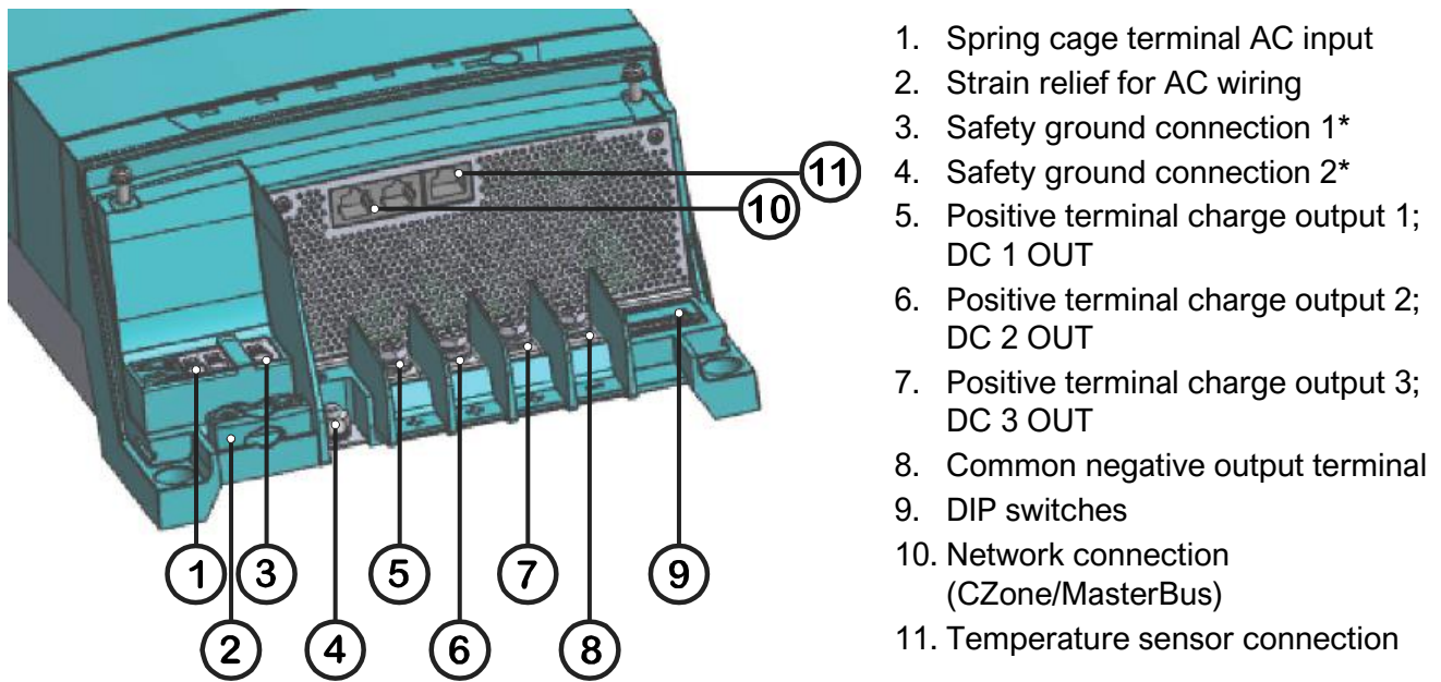
Figure 2: Connections
