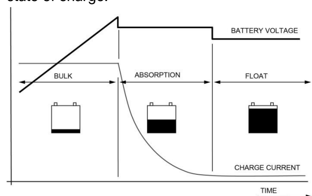
Figure 6: charge process
